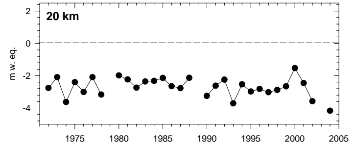
Black Rapids net mass balance
