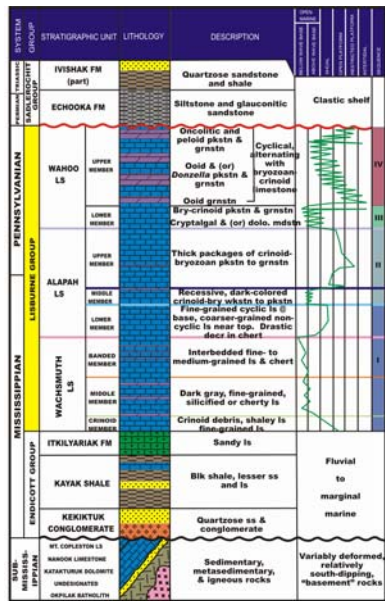
Generalized pre-Mississippian to lower Triassic stratigraphy in the northeastern Brooks Range, including the Carboniferous Lisburne Group. Wahoo data is from the Sadlerochit and Shublik Mountains and Fourth Range (Watts et al., 1995). Wachsmuth and Alapah data is from this study. Figure was modified from Watts et al., 1995.
